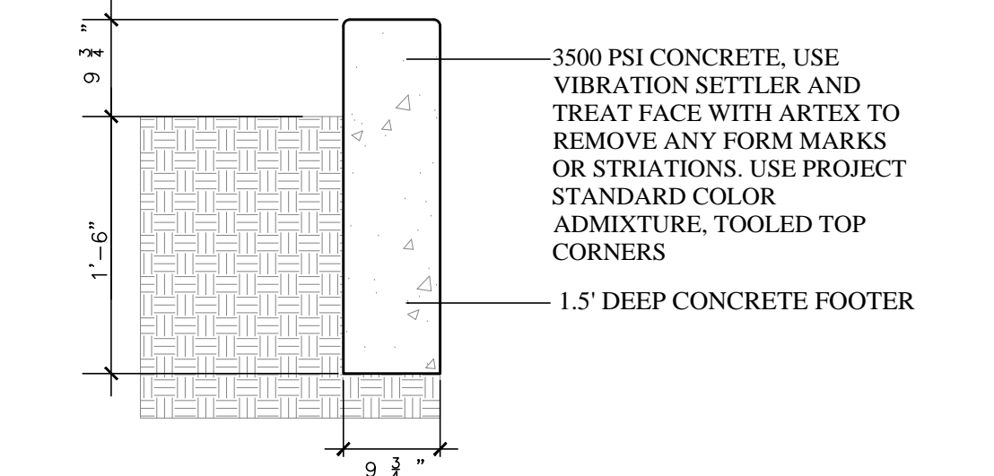
BEE ZONE BOUNDARY MARKERS NO SCALE
